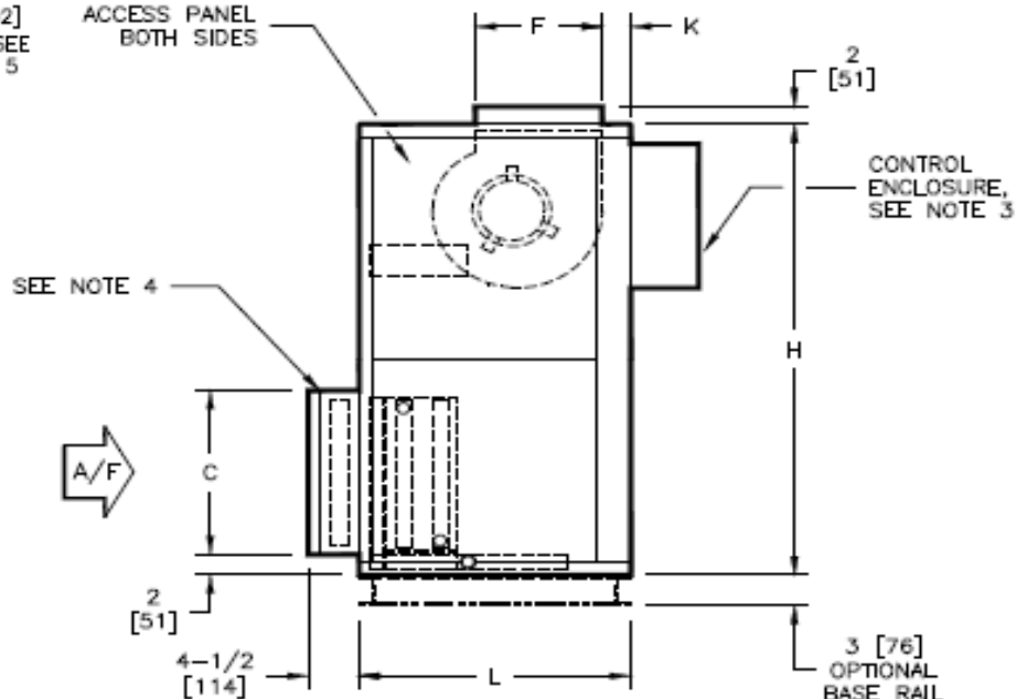
STANDARD FILTER RACK
