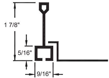
Narrow Tee Detail
