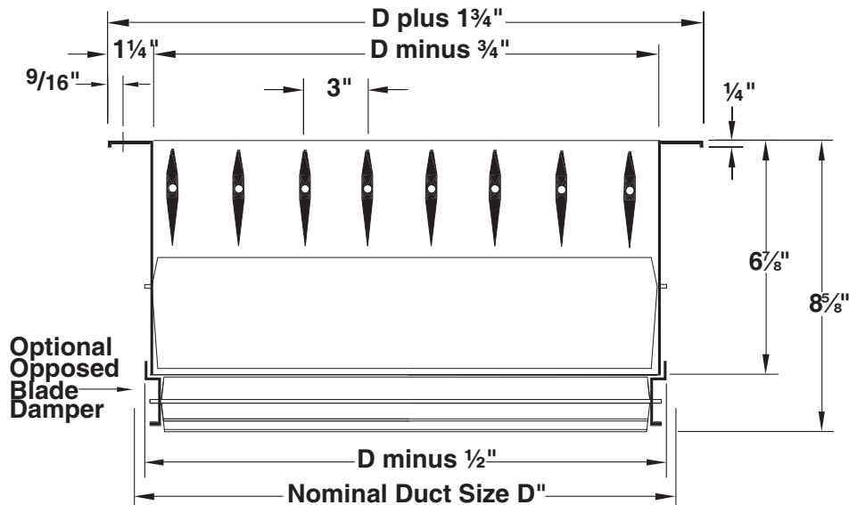
Double Deflection Models: 132RL / 132RS - Border Type 1
