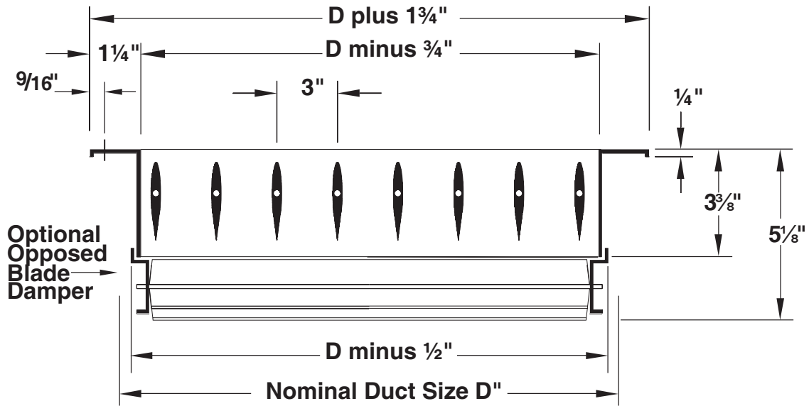
Single Deflection Models: 131RL / 131RS - Border Type 1
