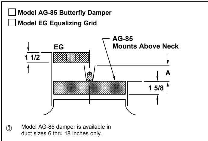
Dimension "A" in Inches, for Dampers Shown
