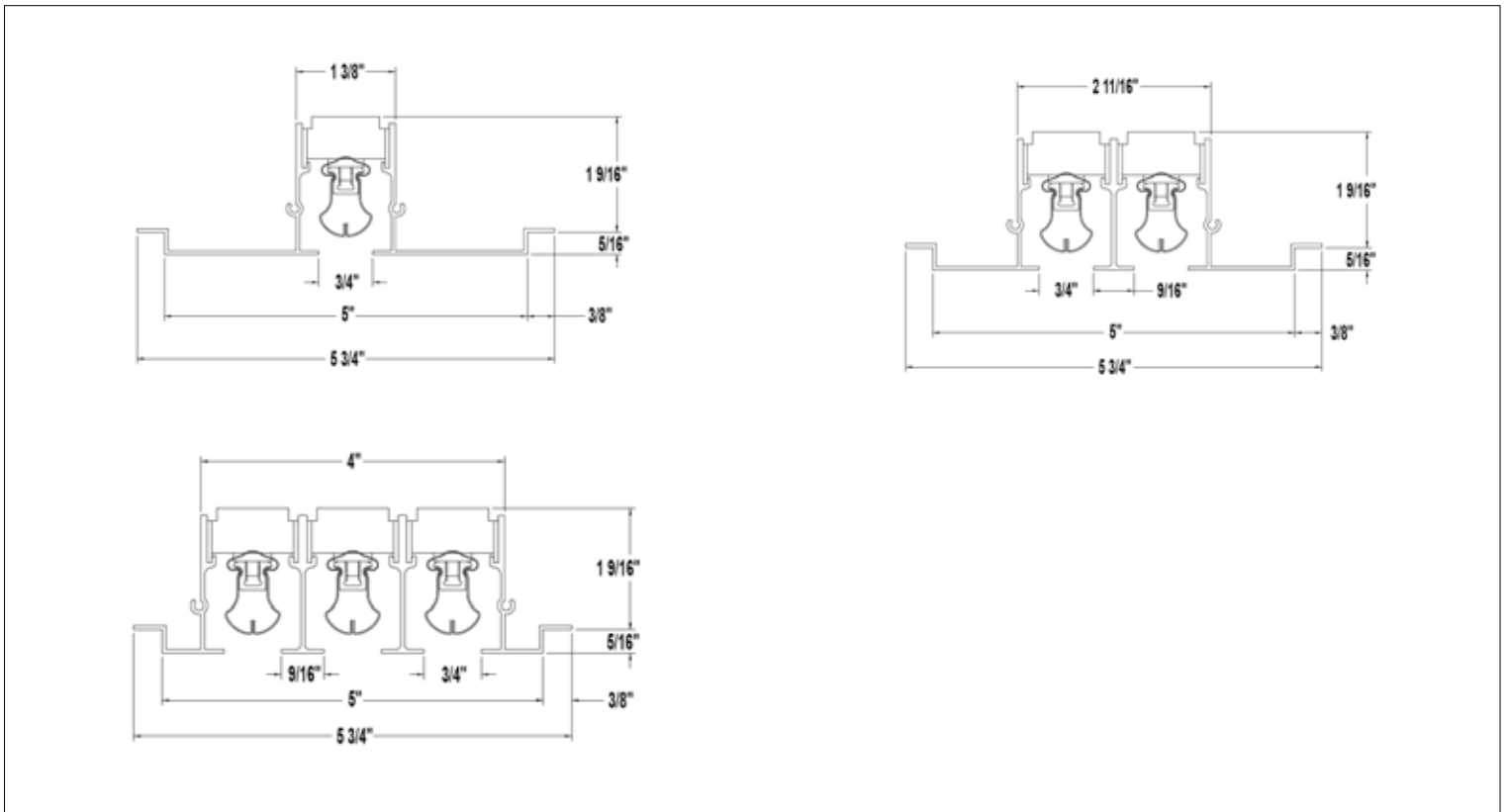
Border Type DF (15/16" Tegular – Drop Face)
