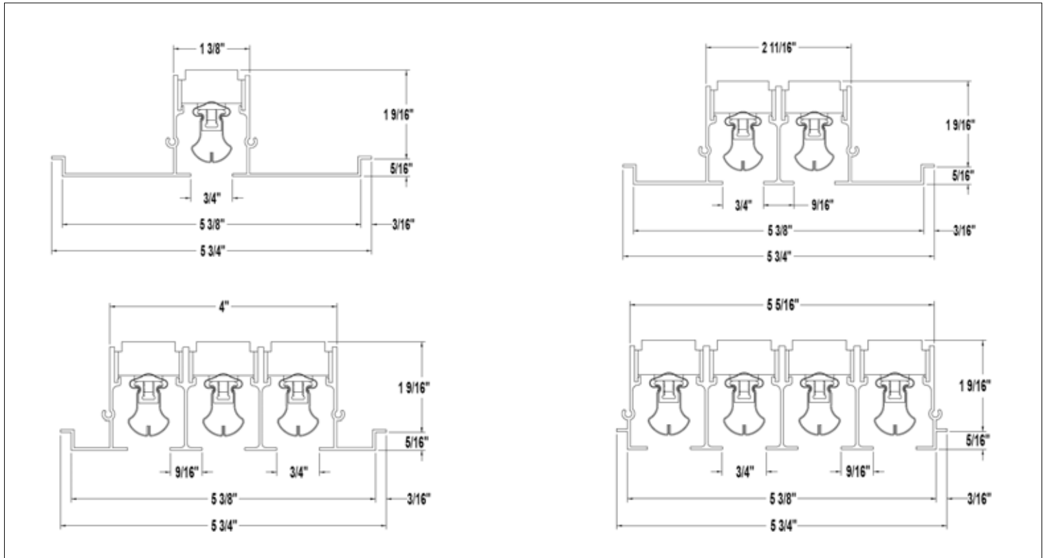
Border Type NT (9/16" Narrow Tee)
