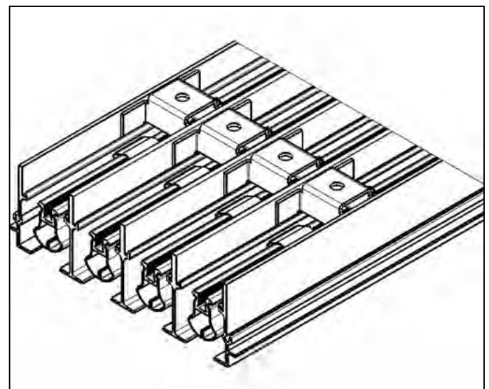
End cap not shown
