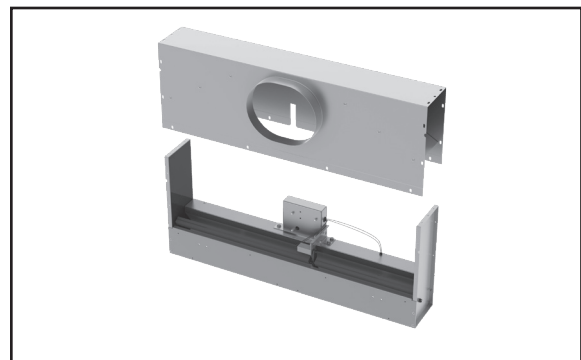
Exploded view of the EOS components
