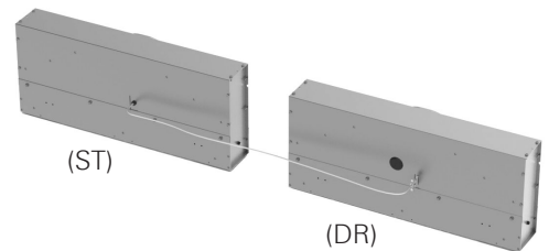
Back view of EOS Primary-Secondary (DR) configuration setup showing cable & dip switch
